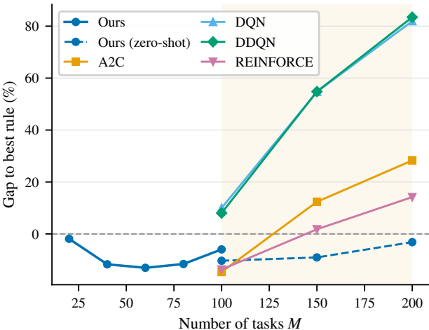
(a) Solution quality across scales
