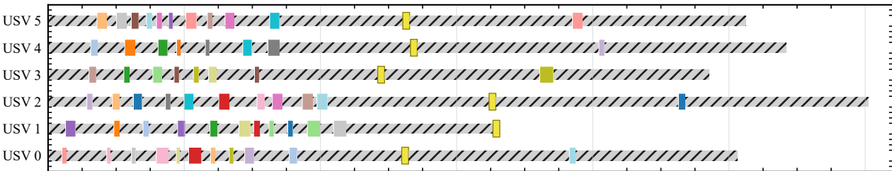
(a) Best rule (MinBattery--NearestTask), C_{\max} = 1204.4
