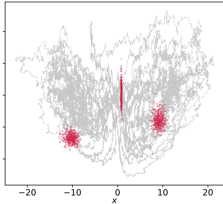
SDE, b = 0.6
