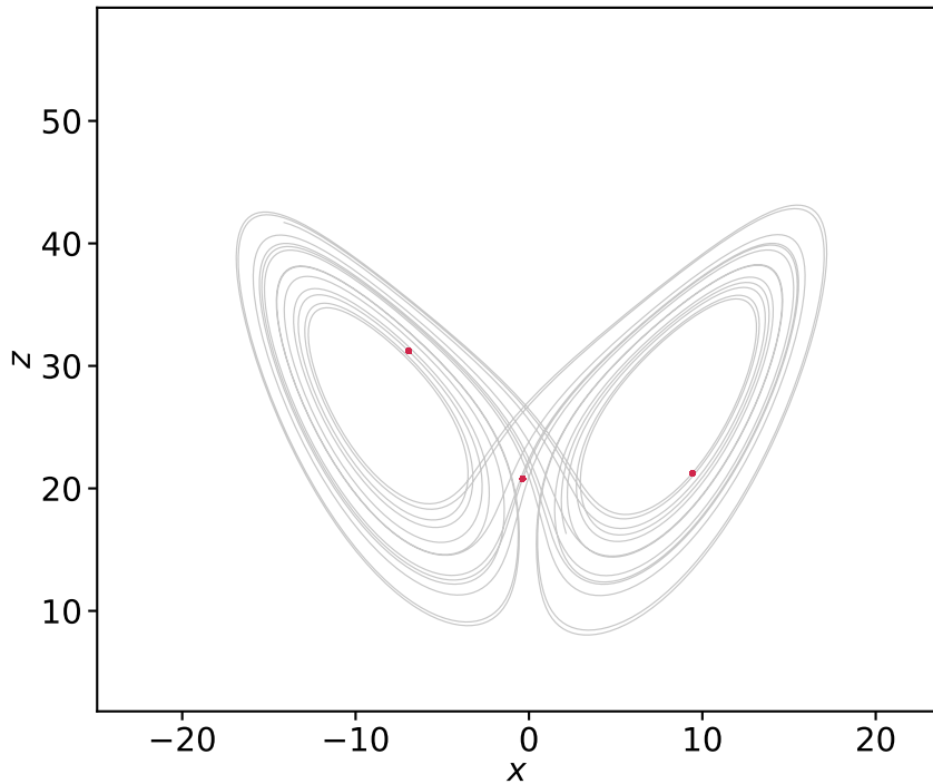
ODE, b = 0
