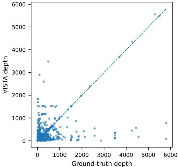
Depth: Ground-truth vs VISTA
