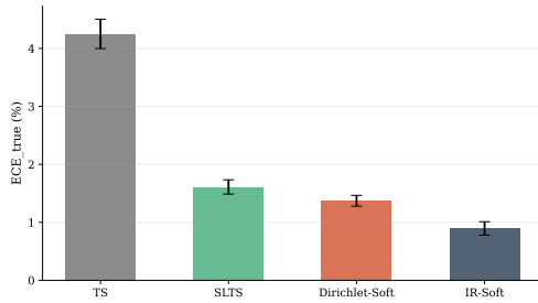
(a) Multi-seed stability. Mean ECE_{\text{true}} ( \pm \text{std} ) over 5 seeds; ranking is stable across splits.
