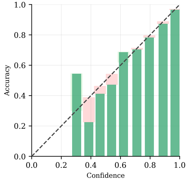
SLTS ECE = 0.5%
