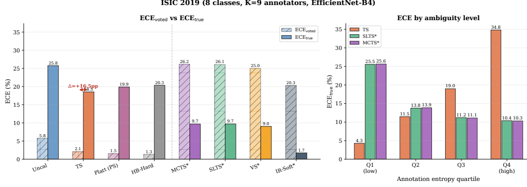
Figure 4: ISIC 2019 results (inspired by the Liu et al. [2020] reader study). Left: ECE_{\text{voted}} vs. ECE_{\text{true}} : voted-label baselines show a large calibration gap; soft-label methods reduce ECE substantially. Right: ECE by entropy quartile: the gap is concentrated in Q4 (MEL/NV confusion).
