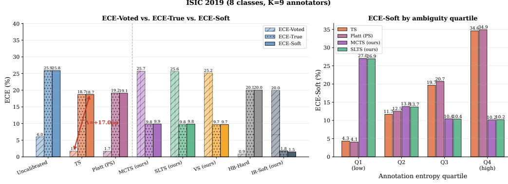
Figure 4: ISIC 2019 calibration results. Left: \text{ECE}_{\text{voted}} vs. ECE: voted-label baselines show a large calibration gap; soft-label methods reduce ECE substantially. Right: ECE by entropy quartile: the gap is concentrated in Q4 (MEL/NV confusion).
