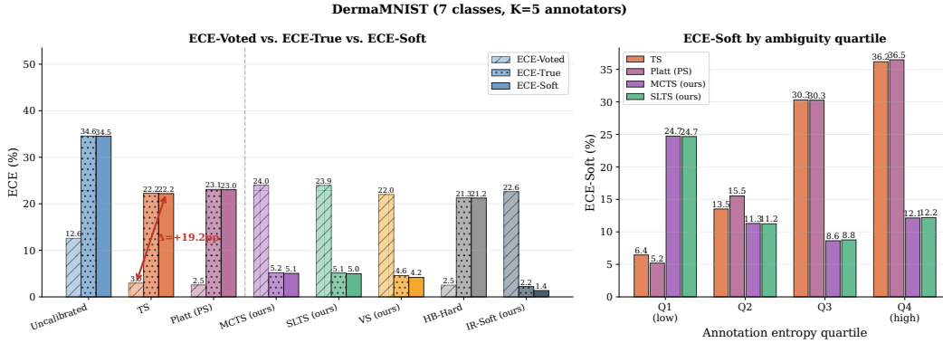
Figure 6: DermaMNIST calibration results. Left: \text{ECE}_{\text{voted}} vs. ECE; right: ECE by entropy quartile. The gap is largest in Q4 (Mel↔NV confusion region).
