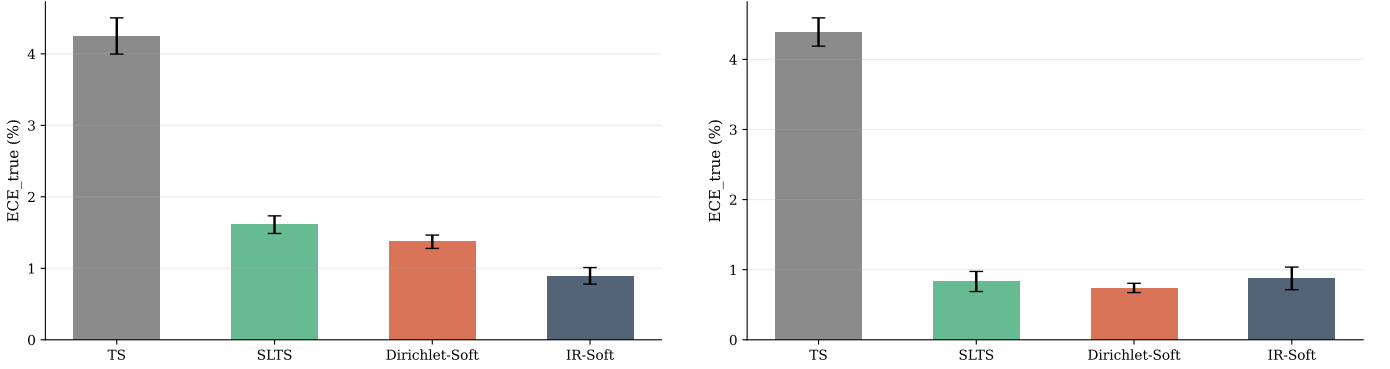
Fig. 15: Multi-seed bar charts — CIFAR-10H. Left: ResNet-50. Right: ViT-B/16.
