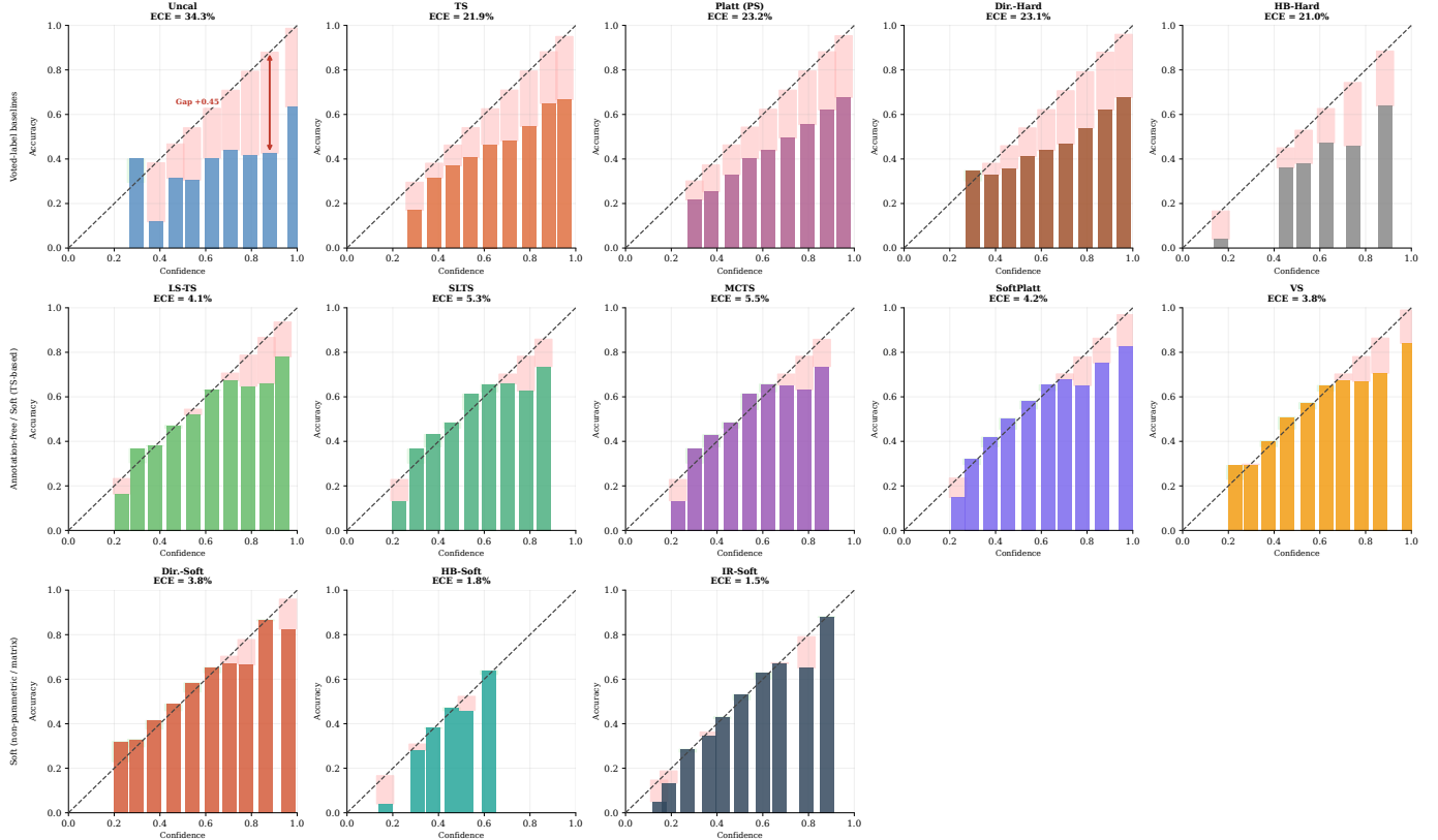
Fig. 31: Reliability diagrams (all methods) — DermaMNIST ResNet-18 (ECE true ).
