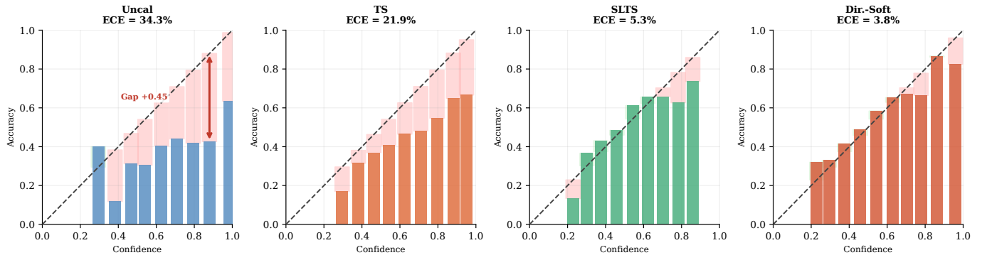
Fig. 29: Reliability diagrams (summary) — DermaMNIST ResNet-18.
