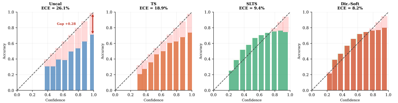
Fig. 25: Reliability diagrams (summary) — ISIC 2019 EfficientNet-B4.
