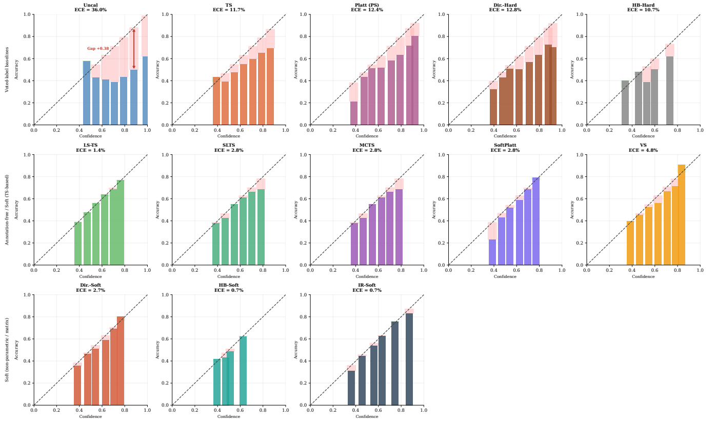
Fig. 24: Reliability diagrams (all methods) — ChaosNLI DeBERTa-v3-base ( ECE_{true} ).
