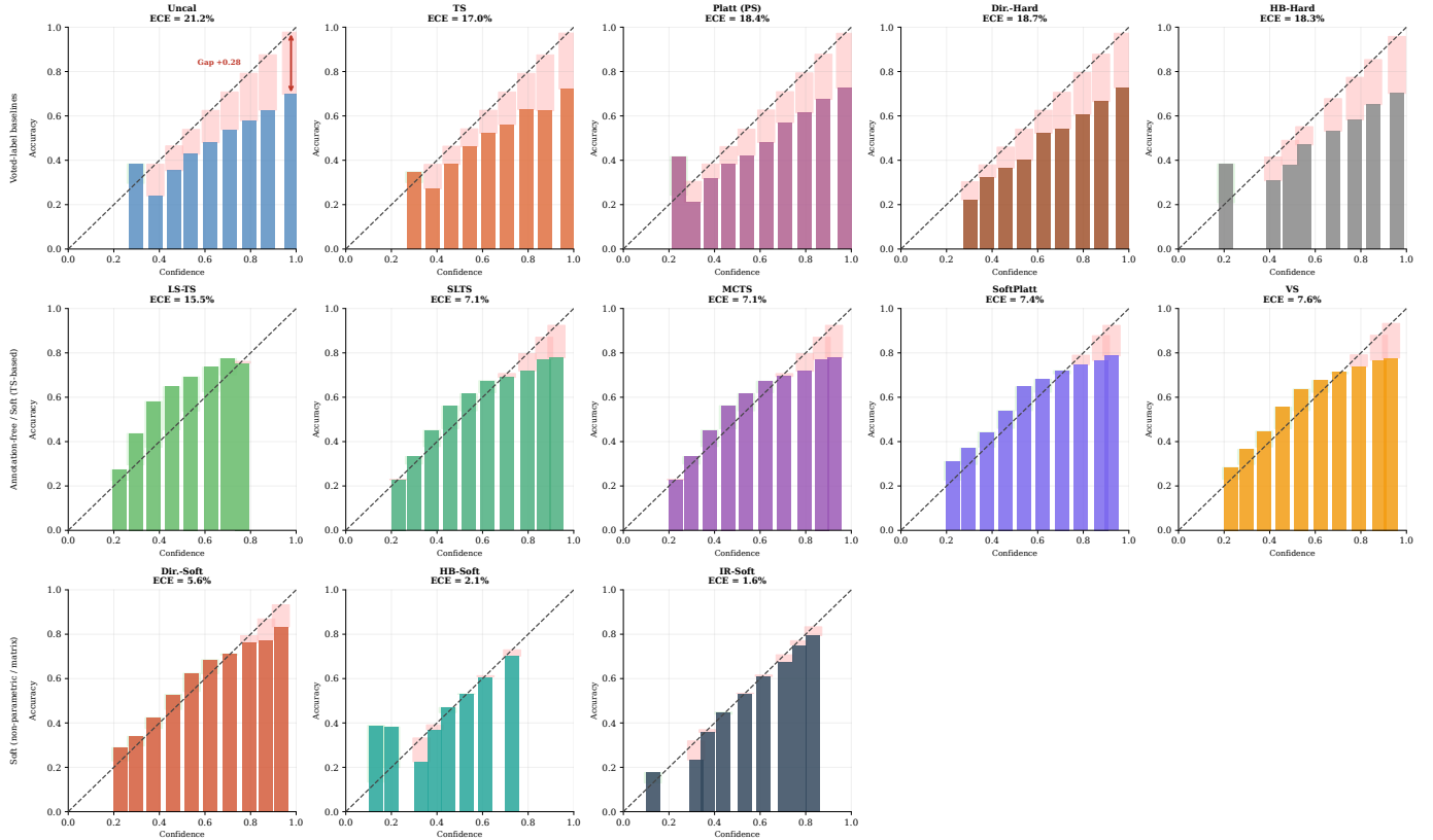
Fig. 28: Reliability diagrams (all methods) — ISIC 2019 ViT-S/16 ( ECE_{true} ).
