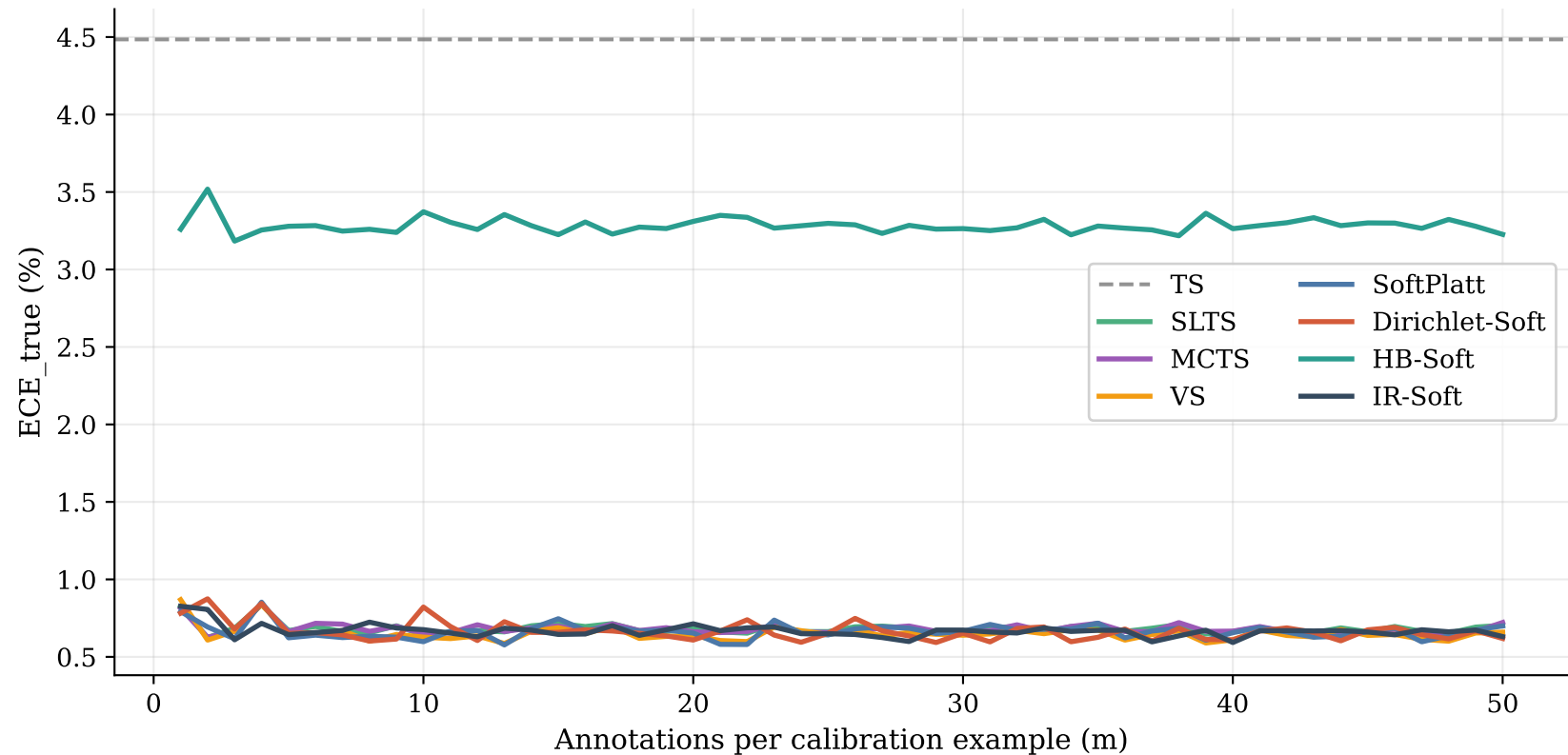
Annotation-count ablation on CIFAR-10H
