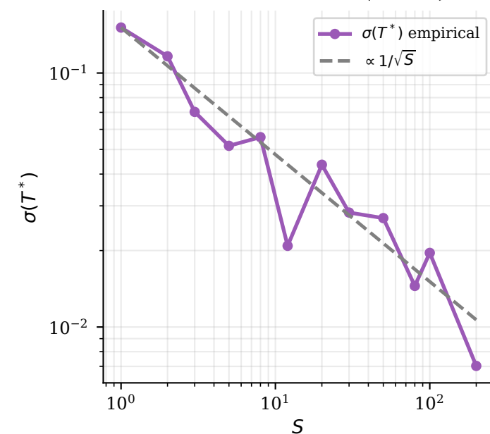
Variance Reduction ( \propto 1/\sqrt{S} )
