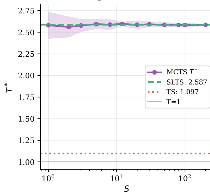
Temperature T^* vs. S
