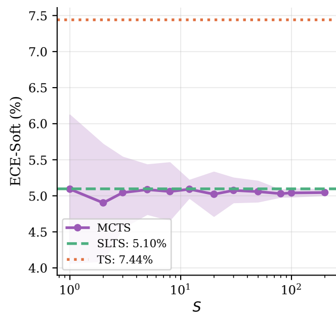
ECE-Soft vs. S
