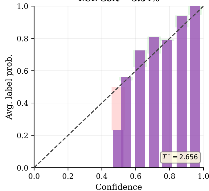
MCTS S=5 ECE-Soft = 5.54%
