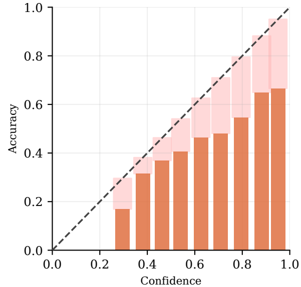
TS ECE = 21.9%
