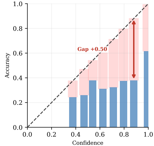
Uncal ECE = 37.7%
