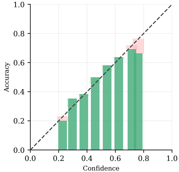
SLTS ECE = 3.1%
