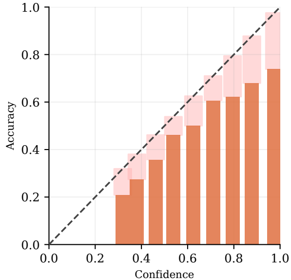
TS ECE = 18.9%
