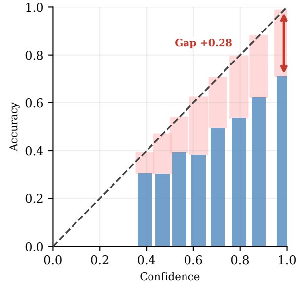
Uncal ECE = 26.1%
