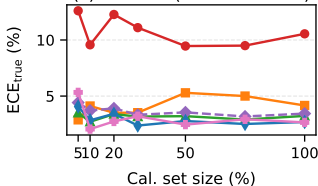
(c) Cal-size (NLI RoBERTa-L)
