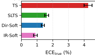
(a) Multi-seed (C10H R50, 5 seeds)
