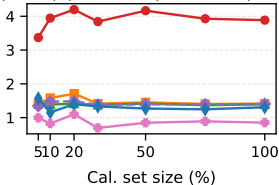
(b) Cal-size (C10H R50)
