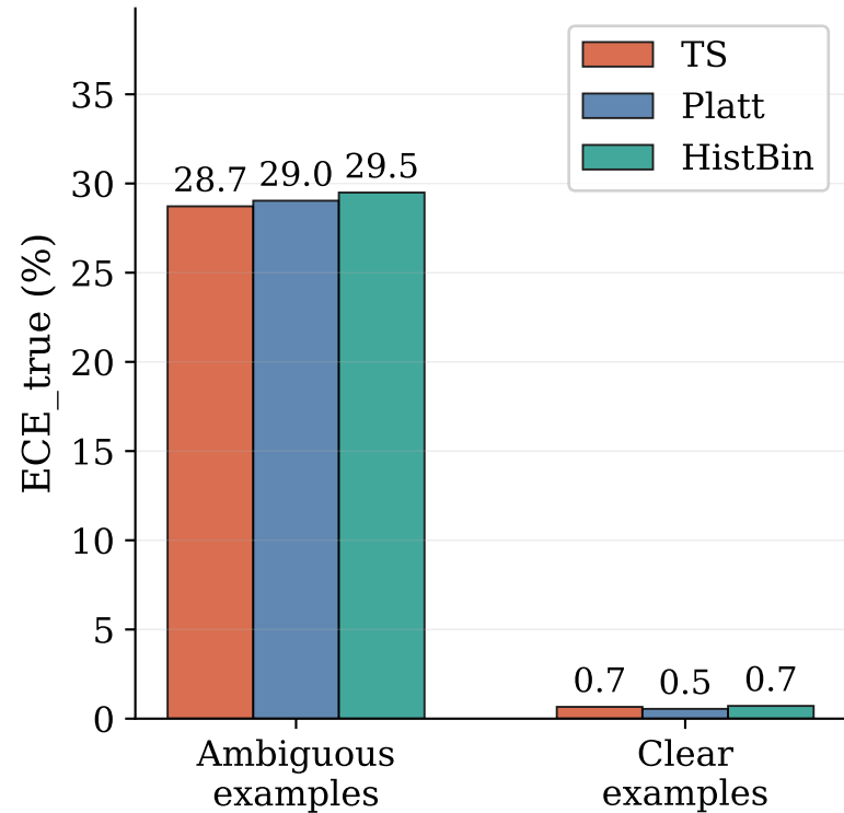
(c) Stratified ECE
