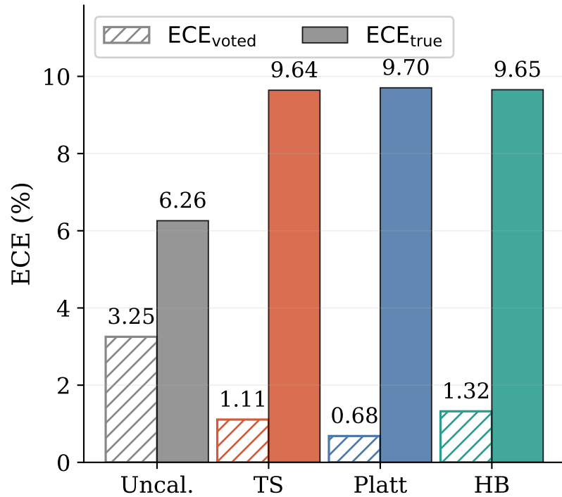
(b) ECE summary
