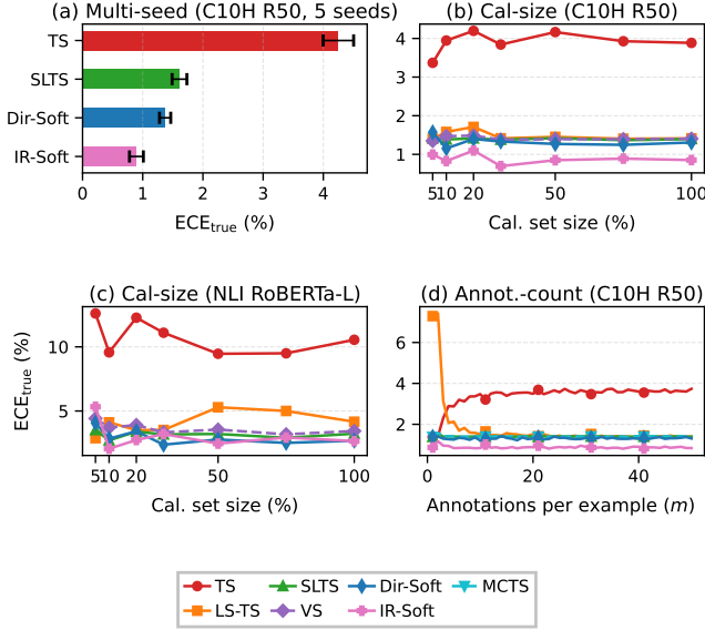
Fig. 9: Robustness of ambiguity-aware calibration. (a) Multi-seed stability (CIFAR-10H R50, 5 seeds). (b)–(c) ECE_{\text{true}} vs. calibration set size on CIFAR-10H R50 and ChaosNLI RoBERTa-L. (d) ECE_{\text{true}} vs. annotation count (CIFAR-10H R50). Rankings are stable across seeds, cal-set sizes, and annotation counts. Full results for all benchmarks are in Appendices G, E, and F.
