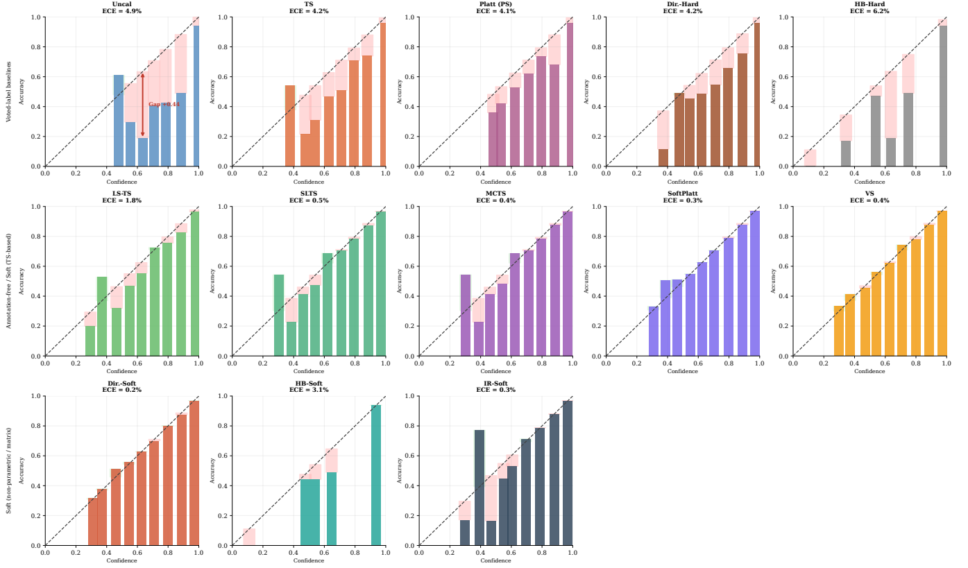
Fig. 21: Reliability diagrams (all methods): CIFAR-10H ViT-B/16 ( ECE_{true} ).
