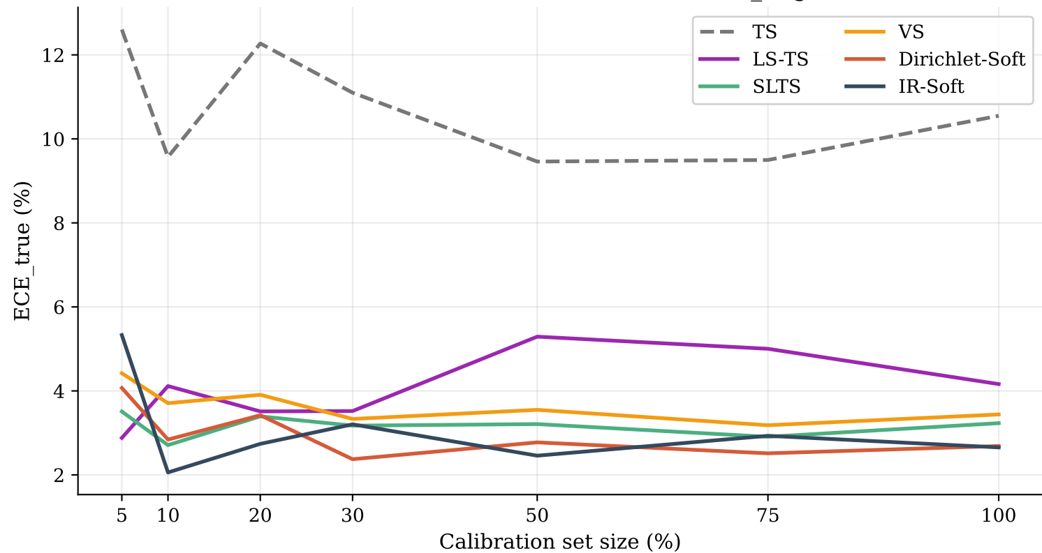
Cal-set-size ablation — chaosnli (roberta_large)
