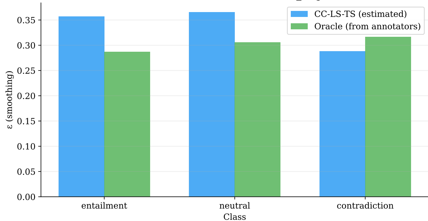
Per-class \varepsilon — chaosnli (roberta_large)
