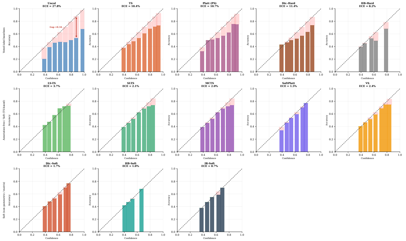
Fig. 23: Reliability diagrams (all methods) — ChaosNLI RoBERTa-Large ( ECE_{\text{true}} ). NLI models are severely overconfident before calibration; ambiguity-aware methods substantially correct this.
