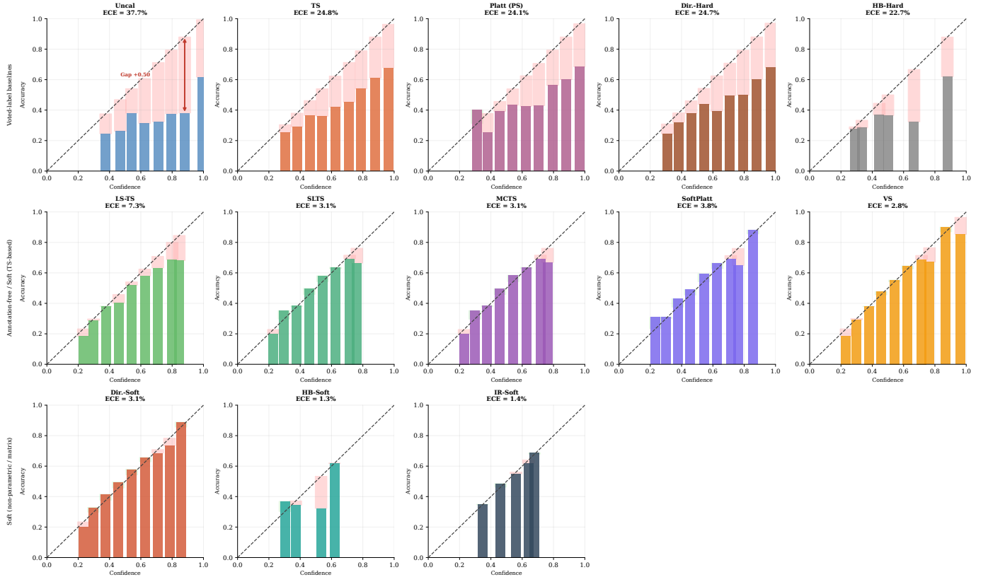
Fig. 32: Reliability diagrams (all methods) — DermaMNIST ViT-S/16 ( ECE_{\text{true}} ).
