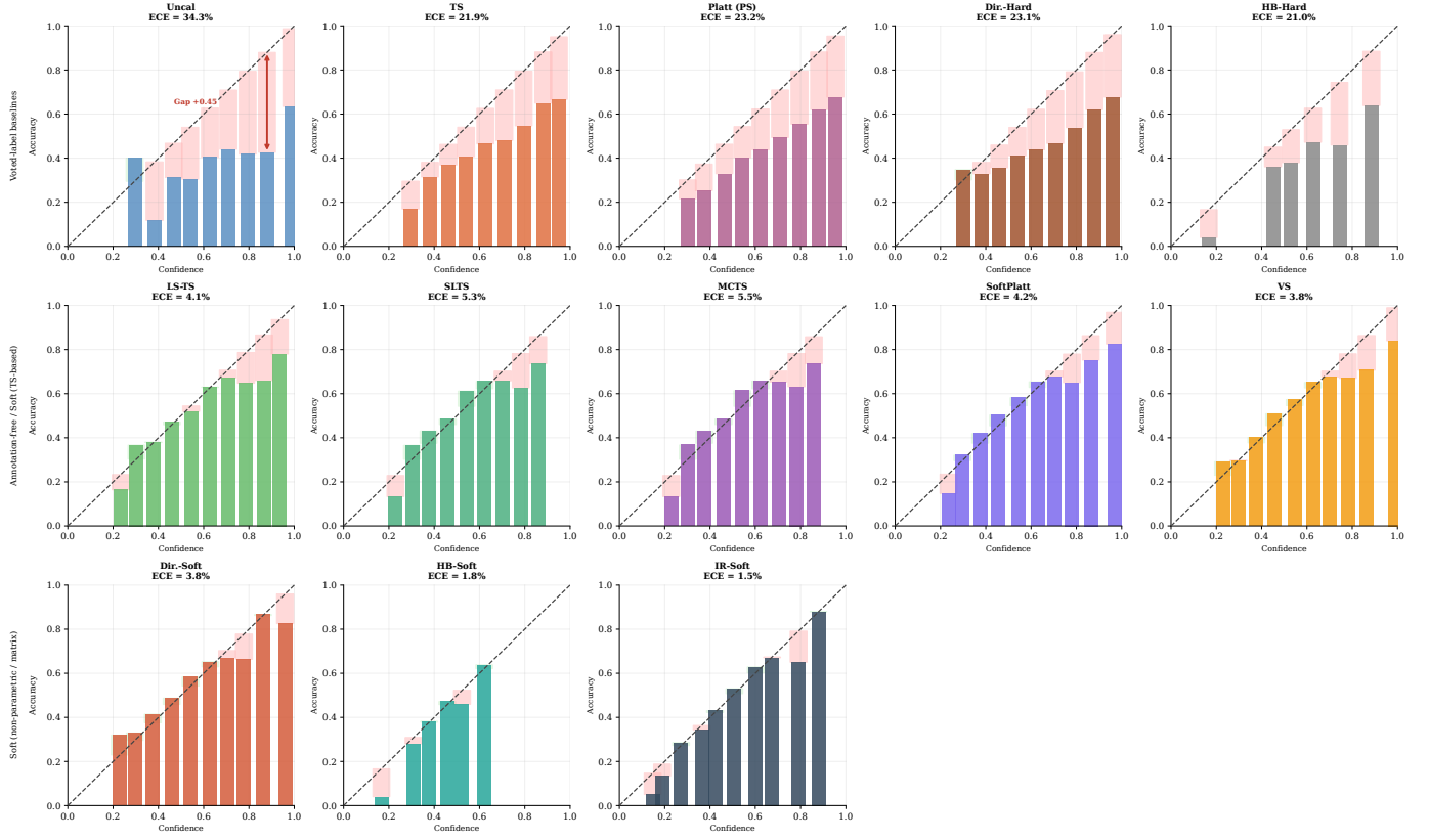
Fig. 31: Reliability diagrams (all methods) — DermaMNIST ResNet-18 ( ECE_{\text{true}} ).
