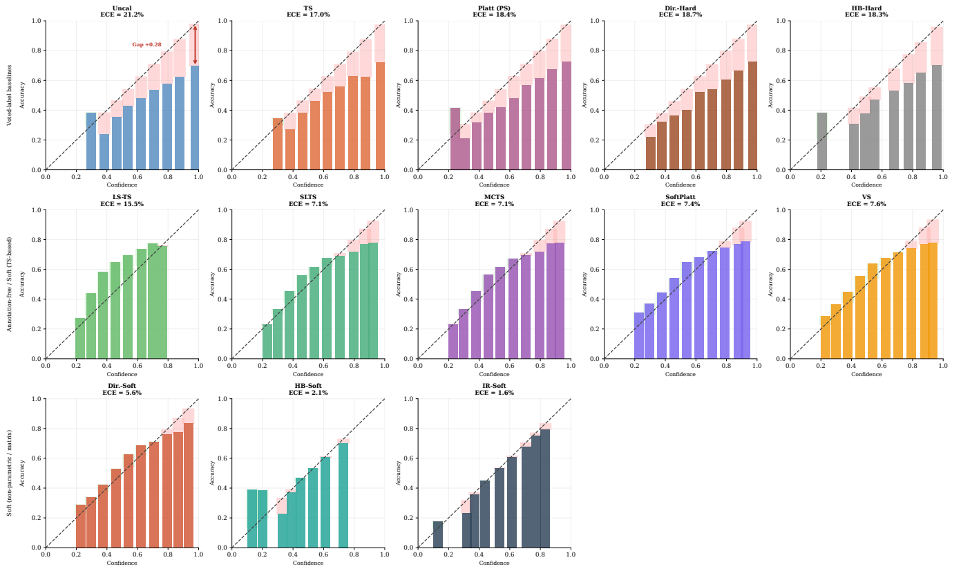
Fig. 28: Reliability diagrams (all methods) — ISIC 2019 ViT-S/16 ( ECE_{\text{true}} ).
