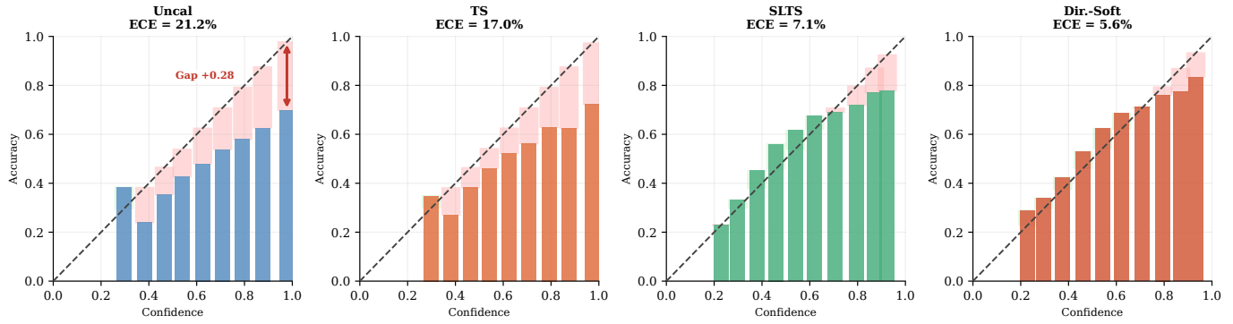
Fig. 26: Reliability diagrams (summary) — ISIC 2019 ViT-S/16.
