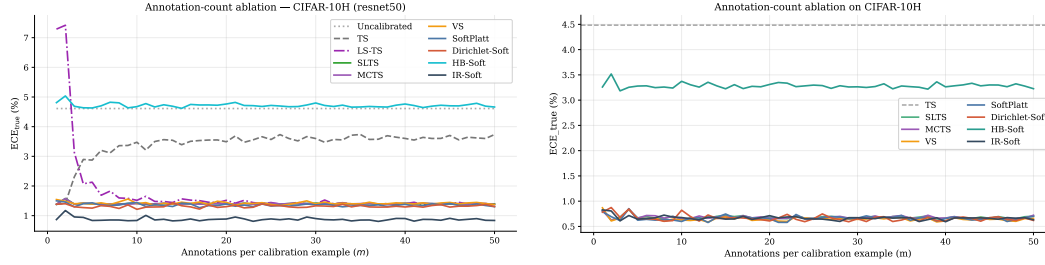
Figure 10: Annotation-count ablation — CIFAR-10H. \text{ECE}_{\text{true}} vs. annotations per image m for ResNet-50 (left) and ViT-B/16 (right). Ambiguity-aware methods are stable for m \geq 2 ; TS rises with m due to target mismatch; LS-TS converges by m \approx 4 .
