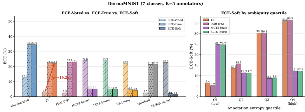
Figure 7: DermaMNIST calibration results. Left: \text{ECE}_{\text{voted}} vs. ECE; right: ECE by entropy quartile. The gap is largest in Q4 (Mel \leftrightarrow NV confusion region).
