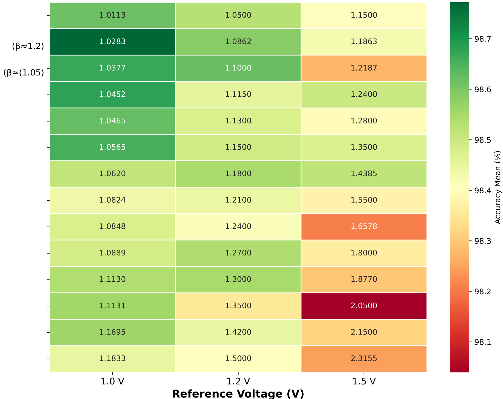
Accuracy Mapping: V_{ref} vs. Overdrive ( \beta ) with sf_p Values
