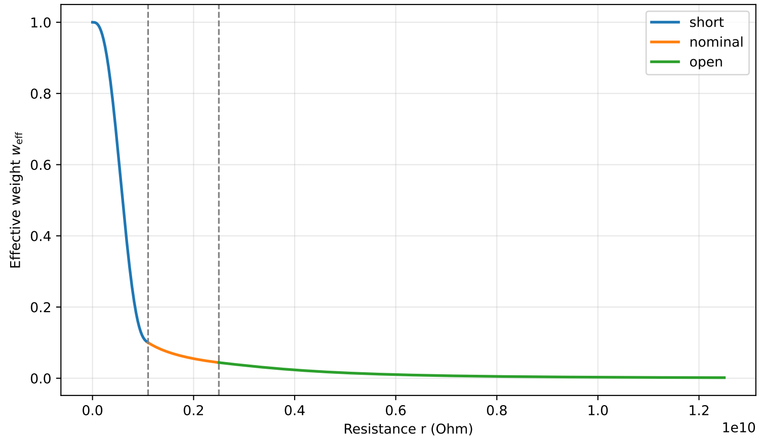
Piecewise mapping from resistance to w_{\text{eff}}
