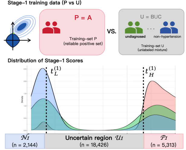
Figure 3. Stage-1 reliable-sample reconstruction using Elastic Net.
