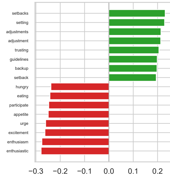
iter 4→5
