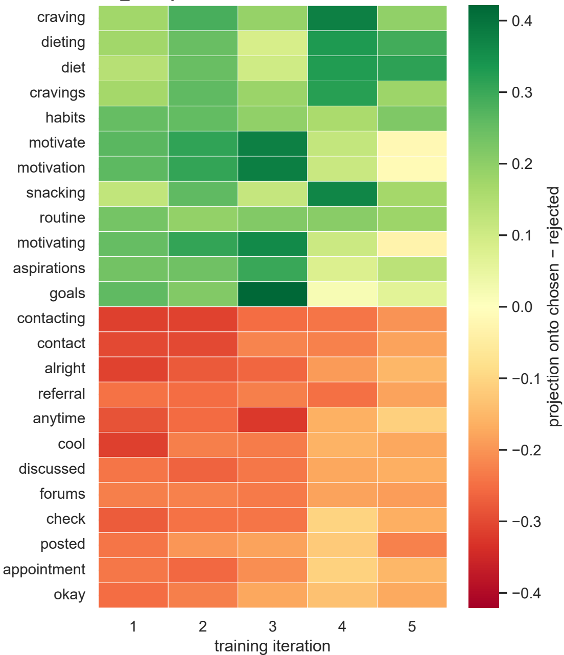
PTO_LA5: preferred-word drift across iterations
