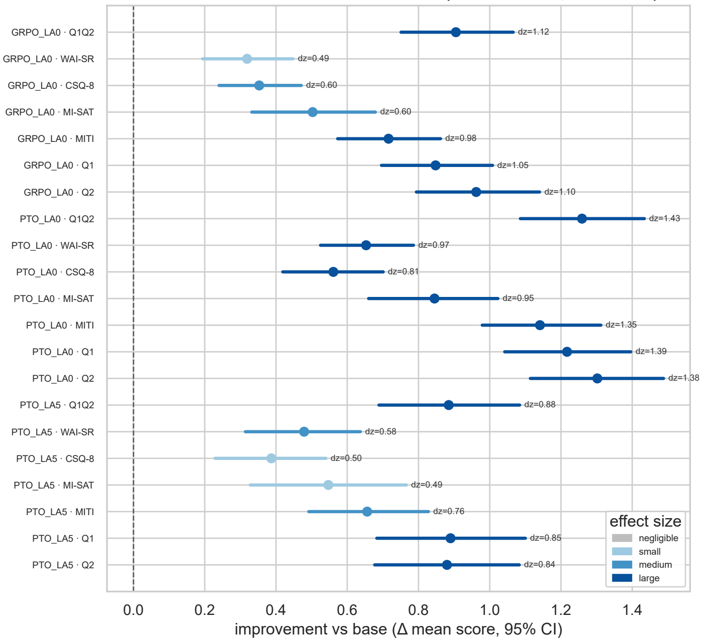
Effect on full-conversation eval vs base (dashed = base; dz labelled)
