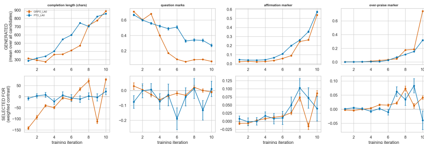
Top: what the policy produces (unweighted mean over every candidate). Bottom: what the update pushes toward within a group (0 = indifferent).
