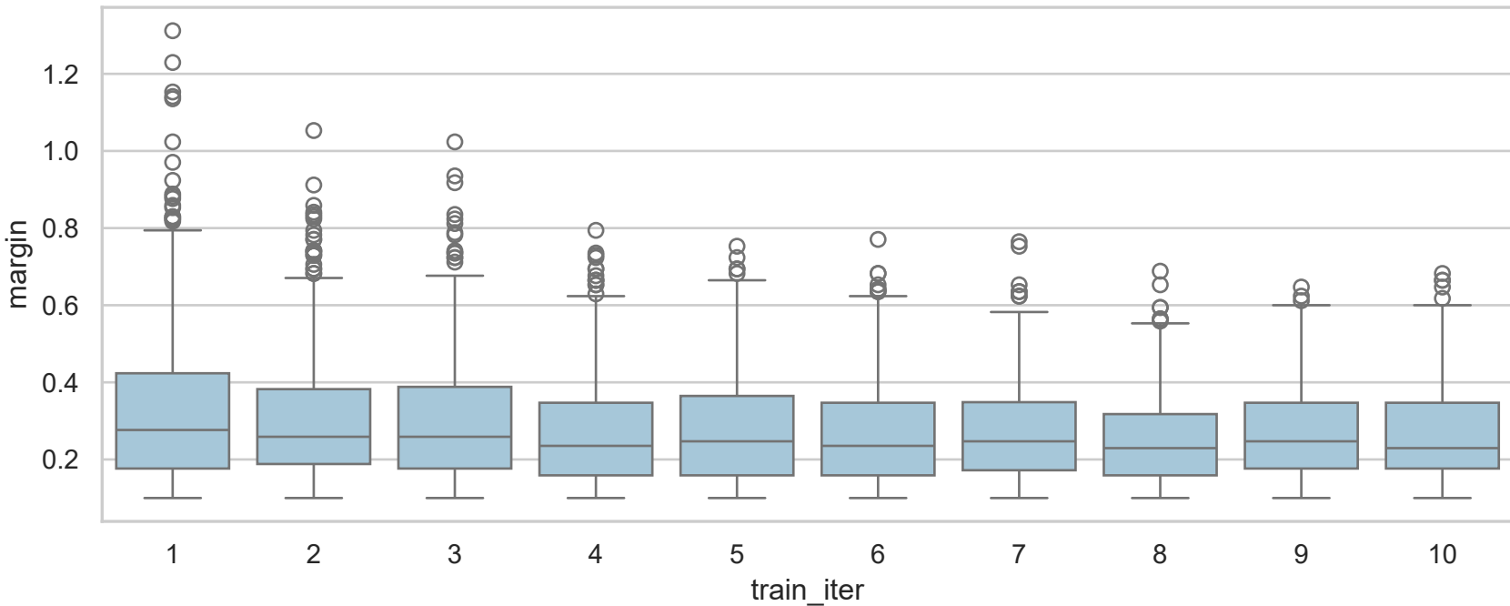
PTO_LA0: PTO chosen-rejected score margin per iteration
