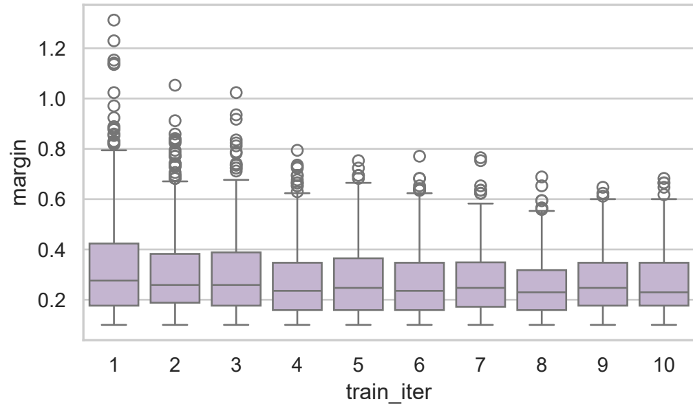
Score margin (chosen - rejected)
