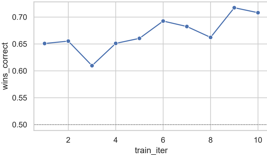
Probe accuracy (chosen > rejected)
