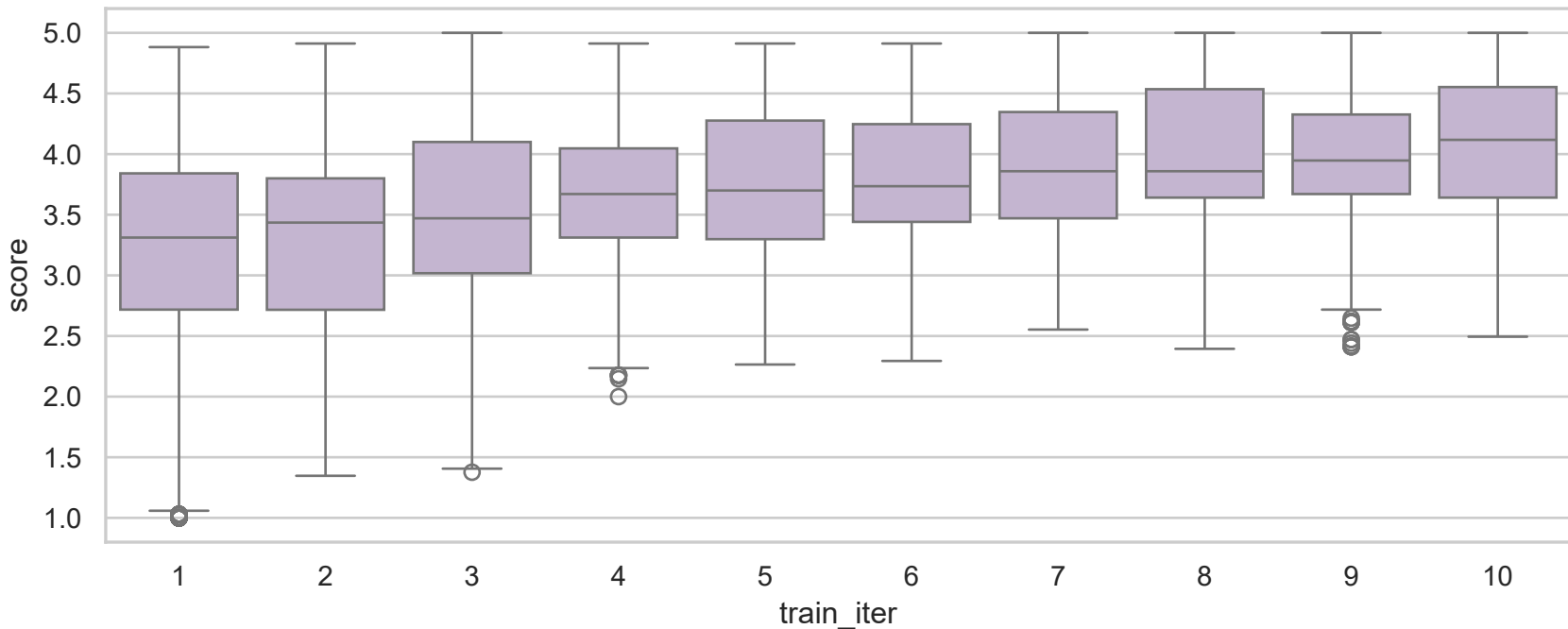
PTO_LA0: candidate reward distribution per training iteration
