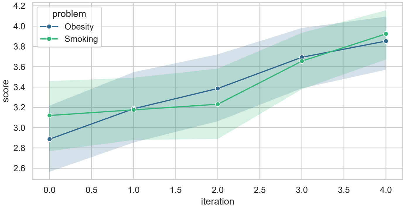
Q1Q2 by problem (true persona) — PTO_LA5
