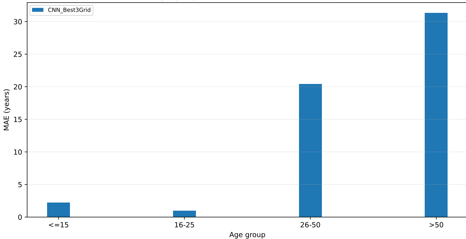
Age-group MAE on the official HHD test split
