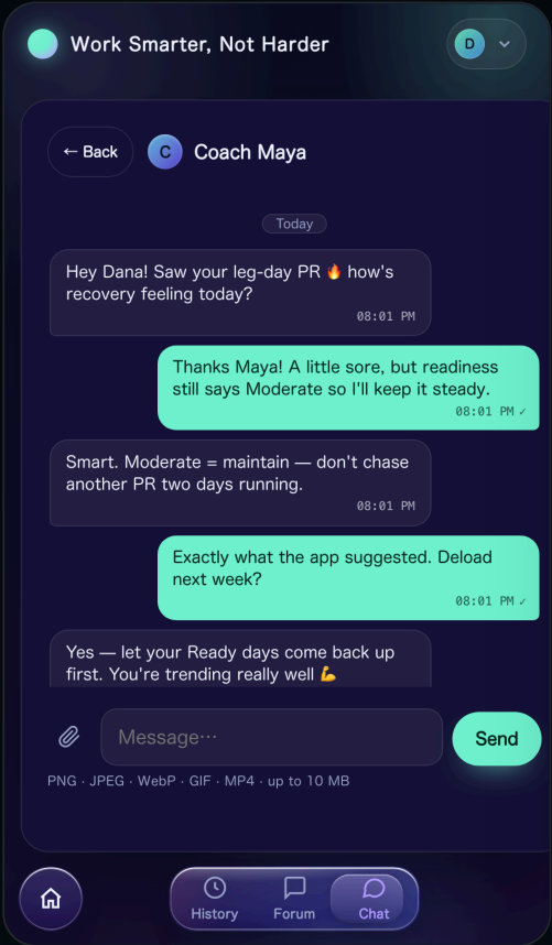
Real-time DMs
