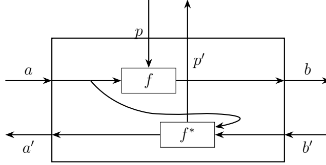
Figure 3.3: ParaLens p\ p'\ a\ a'\ b\ b' : p and p' factored onto the vertical axis.
