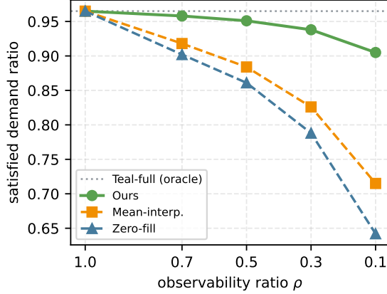
Fig. 4. Satisfied demand ratio versus observability ratio \rho (placeholder data). SiTE stays close to the fully-observed oracle while baselines degrade sharply.
