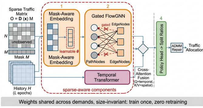
Fig. 3. SiTE overview: a sparse observation is embedded with mask awareness, processed by a gated flow-centric GNN in parallel with a temporal encoder, fused via per-demand cross-attention, and mapped to split ratios refined by ADMM.
