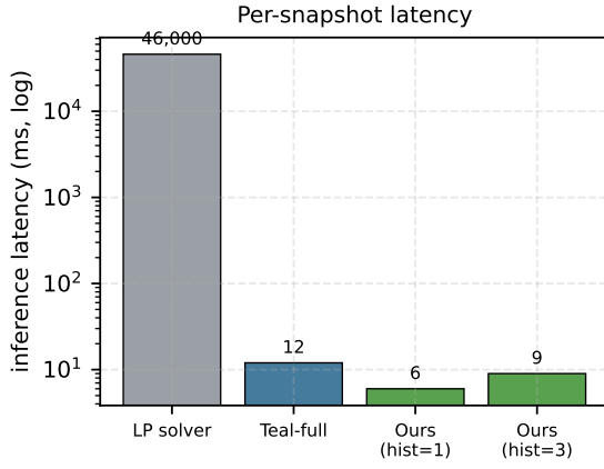
Fig. 9. Per-snapshot inference latency (log scale, placeholder data).
