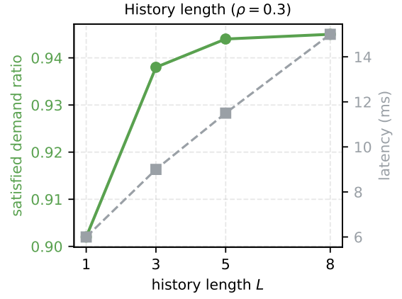
Fig. 11. History-length sweep at \rho = 0.3 (placeholder data): quality saturates while latency grows linearly.
