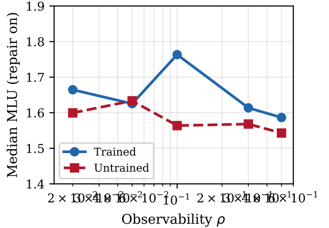
Fig. 4. Trained vs. untrained SiTE with repair enabled. Training yields no measurable gain at any observability level.
