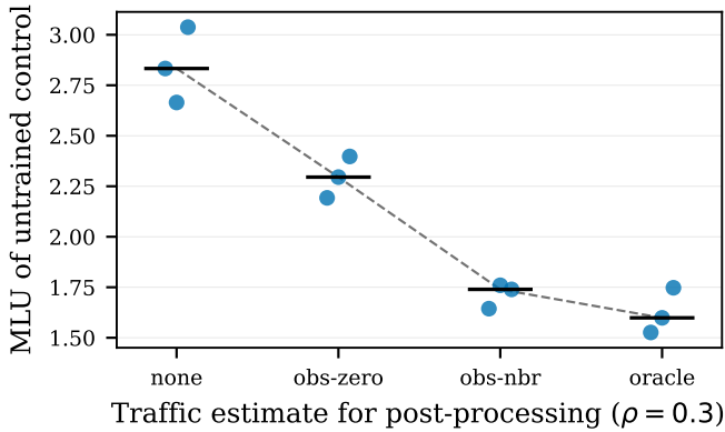
Fig. 7. Sensitivity to the traffic estimate used by post-processing at \rho = 0.3 . Each dot is one experimental repeat; black bars denote medians. The oracle uses unavailable complete traffic and five rounds of ten sweeps; deployed methods use an observation-derived estimate.
