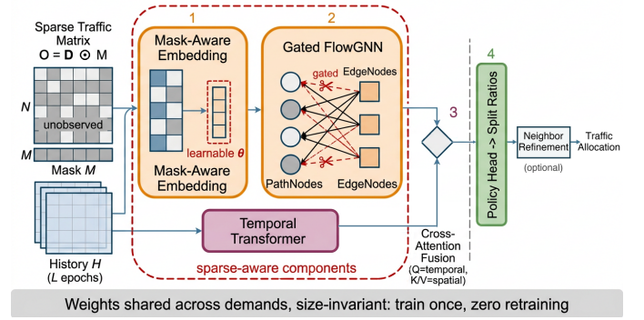
Fig. 3. SpaTE overview. The numbers 1–4 in the figure mark the four stages of Section 4.1: 1 mask-aware demand embedding; 2 mask-gated FlowGNN (Section 4.3); 3 temporal encoding and per-demand cross-attention; and 4 split-ratio prediction. The optional neighbor-assisted refinement uses observation-derived traffic estimates to rebalance paths; it is not ADMM or a projection onto link-capacity constraints.
