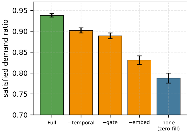
Ablation at \rho = 0.3
