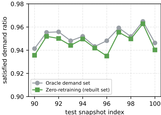
Generalization under demand-set drift
