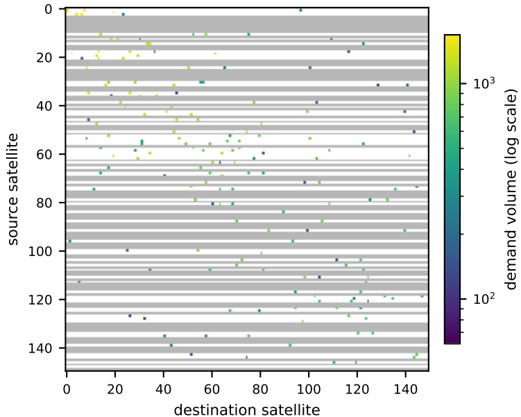
(b) Sparse observation ( \rho = 0.5 , node-level)
