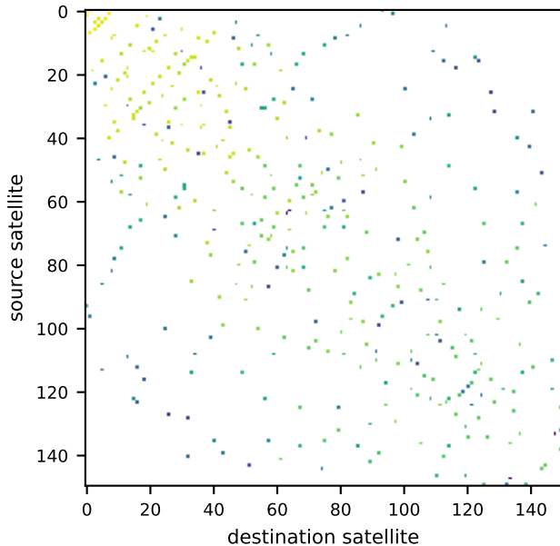
(a) Ground-truth traffic matrix
