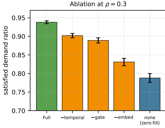
Fig. 8. Component ablation at \rho = 0.3 (placeholder data). Each sparse-aware module contributes to the final performance.
