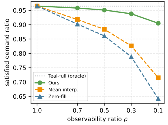
Fig. 6. Satisfied demand ratio versus observability ratio \rho (placeholder data). SiTE stays close to the fully-observed oracle while baselines degrade sharply.
