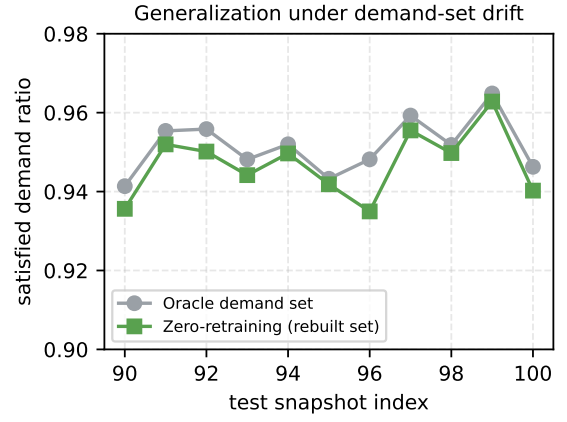
Fig. 10. Per-snapshot satisfied ratio on the test slice (placeholder data): weights trained on the training-slice demand set are reused on the rebuilt test-slice set with negligible loss.
