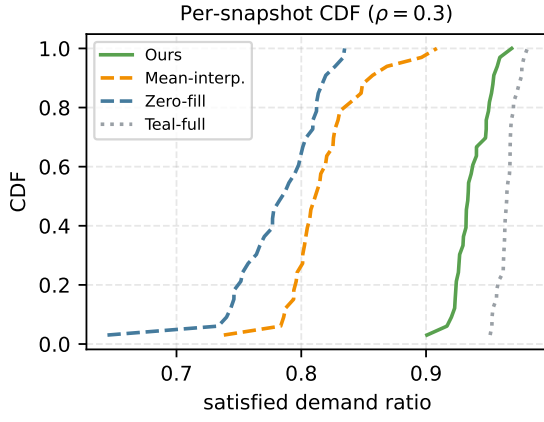
Fig. 5. CDF of per-snapshot satisfied ratio at \rho = 0.3 (placeholder data).
