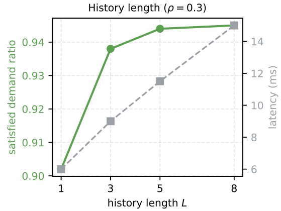
Fig. 13. History-length sweep at \rho = 0.3 (placeholder data): quality saturates while latency grows linearly.
