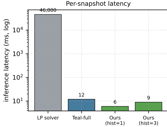
Fig. 11. Per-snapshot inference latency (log scale, placeholder data).
