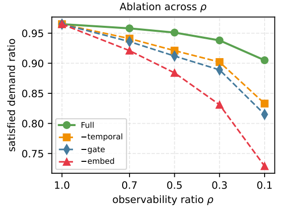
Fig. 7. Ablation across observability ratios (placeholder data). Module contributions grow as observations become scarcer.
