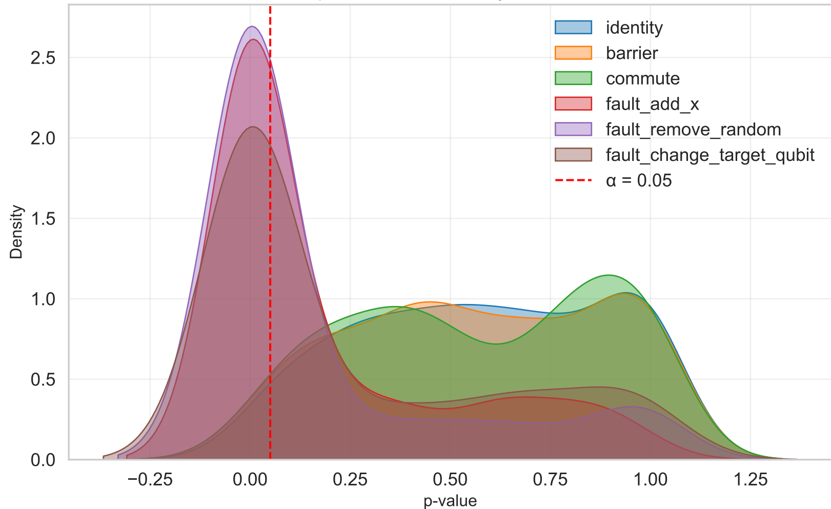
p-value Distribution by Relation
