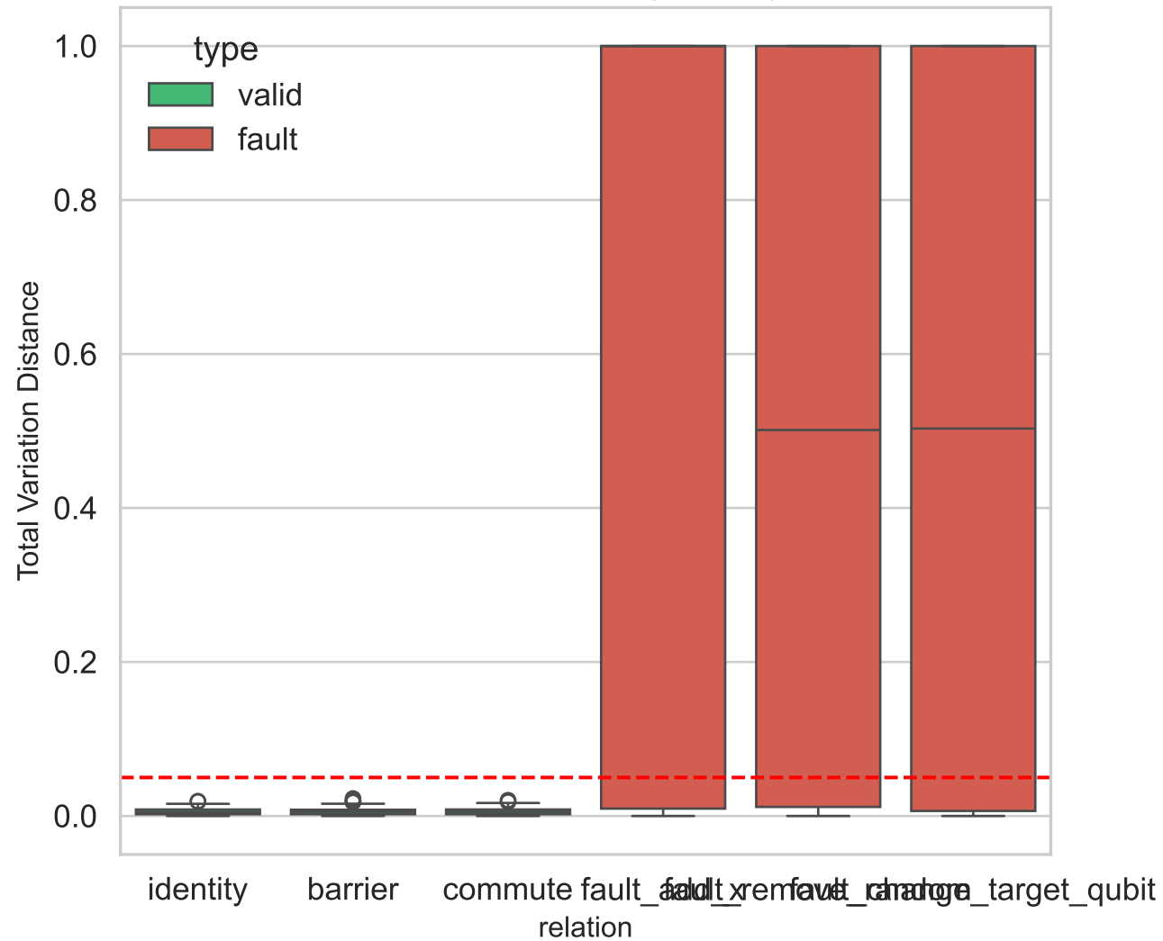
TVD Distribution (Boxplot)
