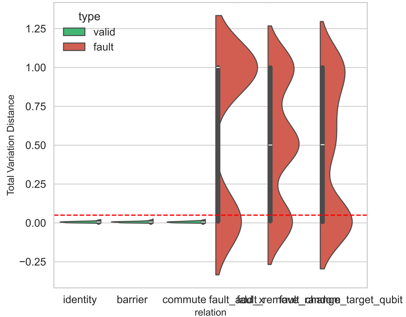
TVD Distribution (Violin)
