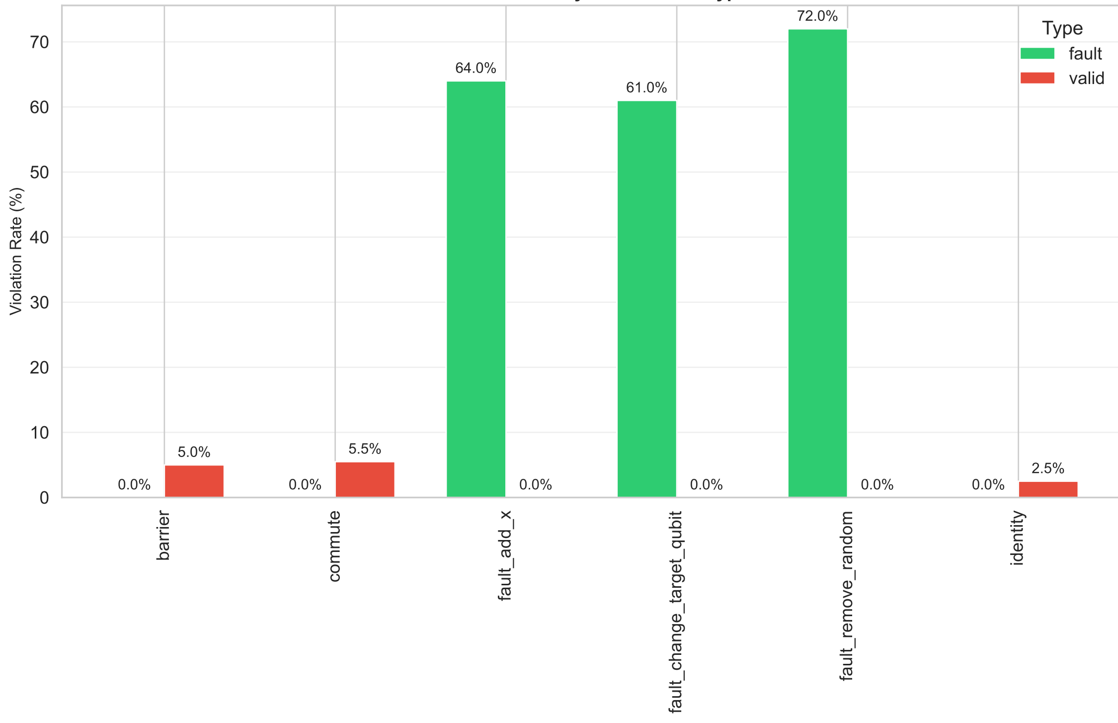
Violation Rate by Relation and Type
