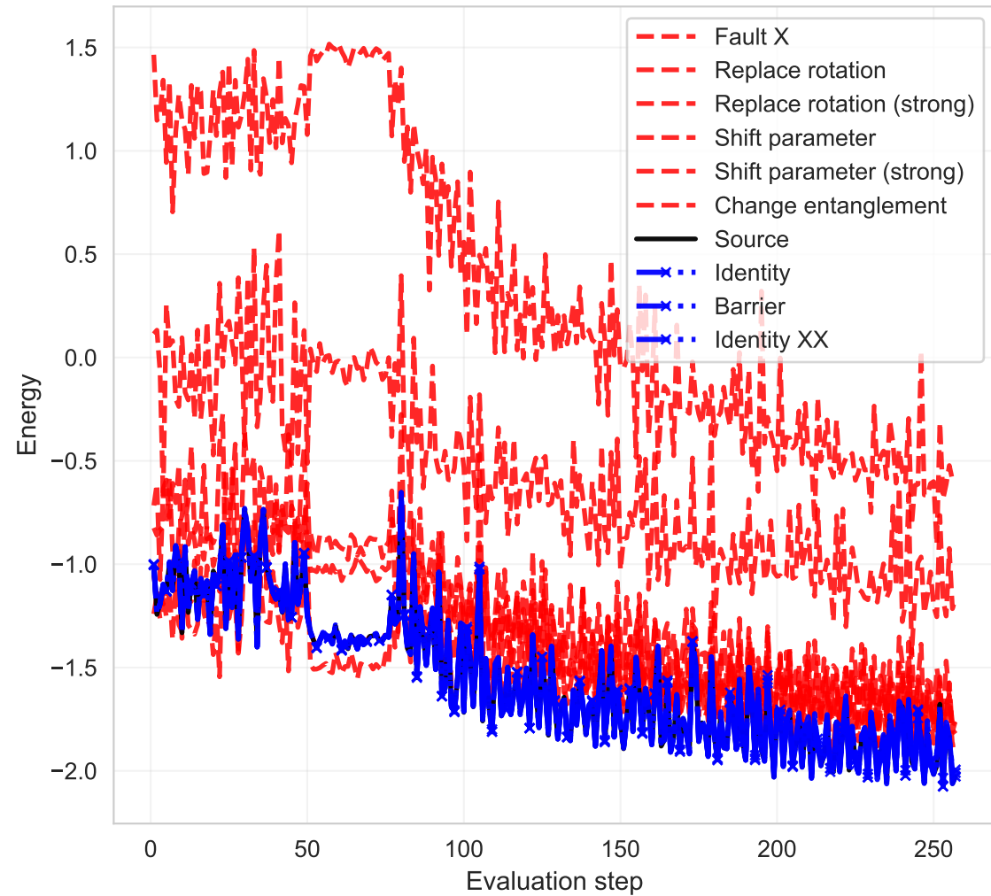
(a) Energy Convergence
