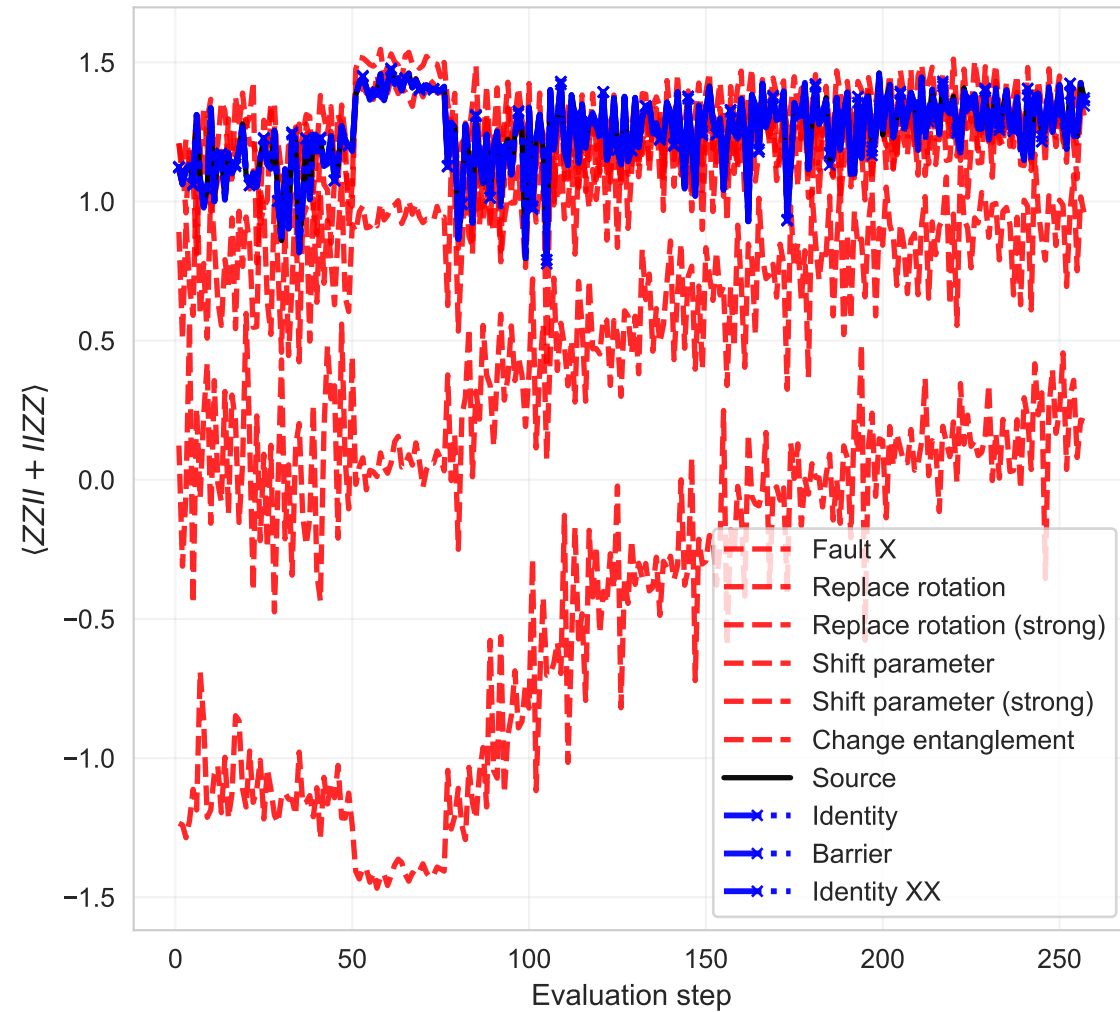
(b) Symmetry Observable Evolution
